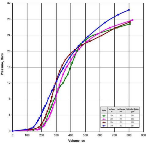
Fig. 2. Pressuremeter test results
